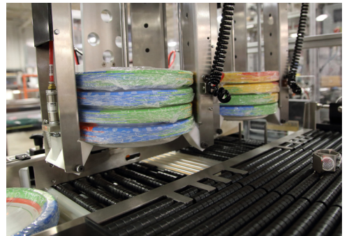
STACKER WITH SLIP-TORQUE SURFACE FOR ROBOTIC CASE PACKER
