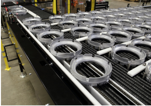
MULTI-LANE TO SINGLE LANE ACCUMULATION
