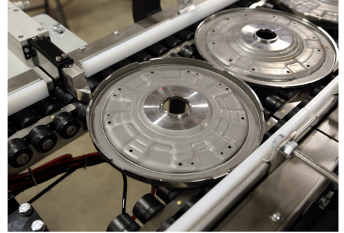
SINGLE LANE ACCUMULATION WITH OPEN CENTER SURFACE
